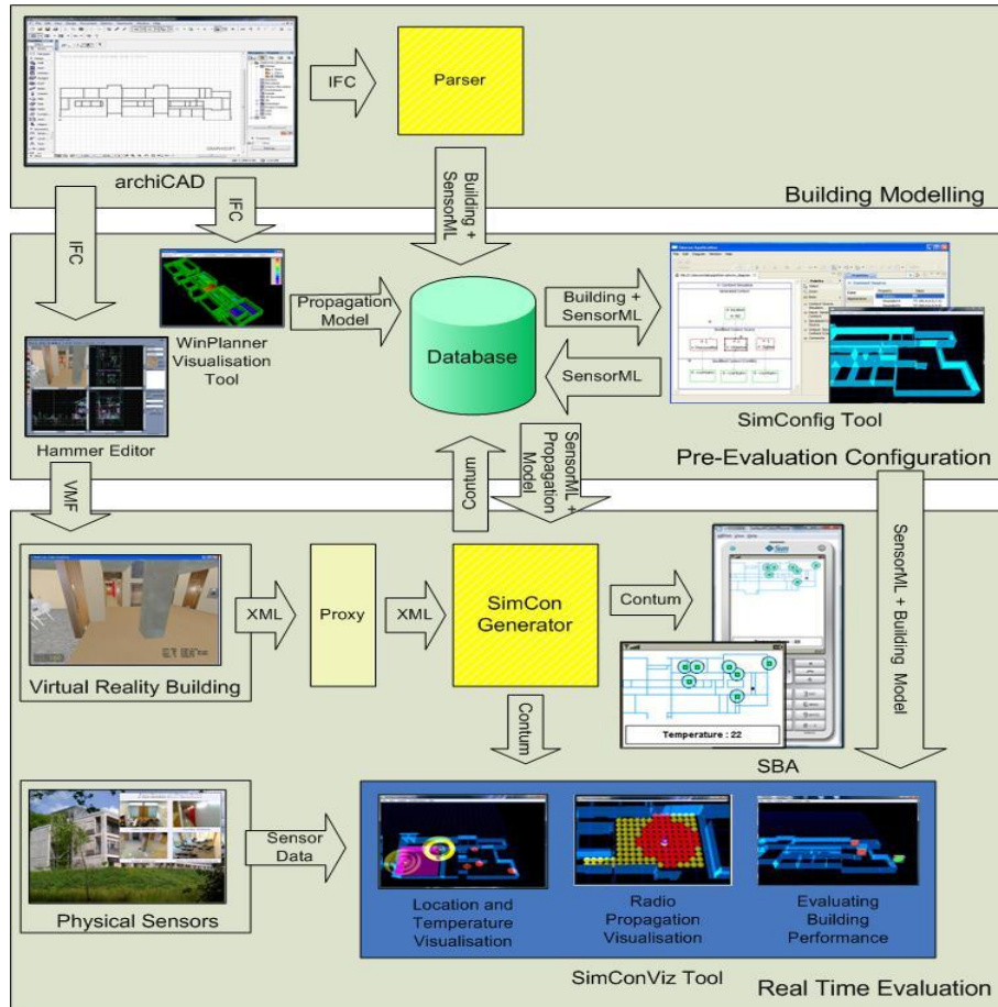
Figure 1 Smart Building Modelling to Support Smart Building Application Evaluation
