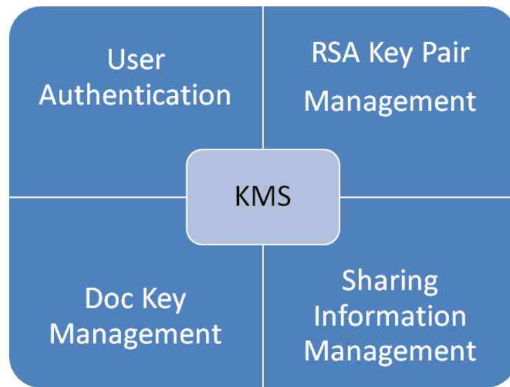
Figure 3.7: KMS Architecture
