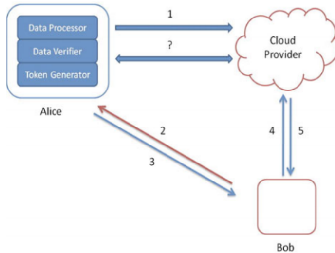
Figure 2.1: Customer Architecture [19]
